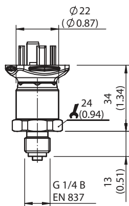
Process connection G 1/4 B according to EN 837 with connection for L-connector according to DIN EN 175301-803 A
