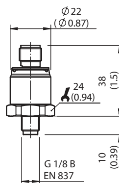
Process connection G 1/8 B according to EN 837 with round connector M12 x 1, 4-pin
