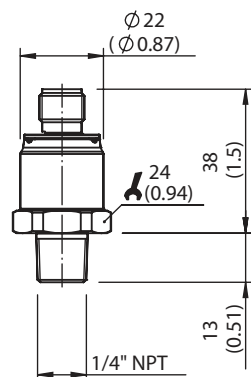
Process connection 1/4" NPT with round connector M12 x 1, 4-pin
