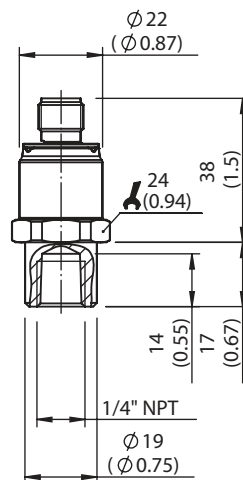
Process connection 1/4" NPT female with round connector M12 x 1, 4-pin
