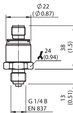
Process connection G 1/4 B according to EN 837 with round connector M12 x 1, 4-pin
