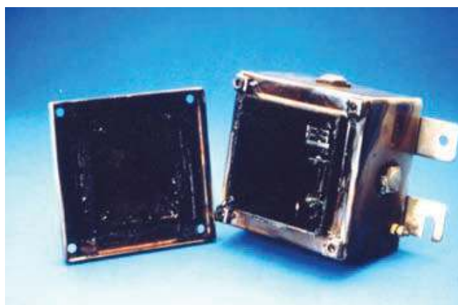
SX Range Enclosure after BS6387 Testing
