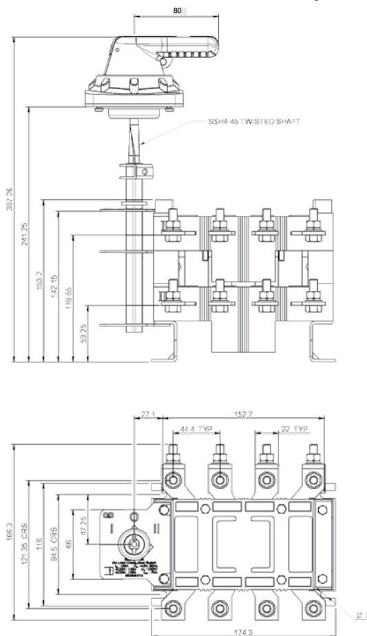
Frame Size C2C - 125A, 160A & 200A Ratings
