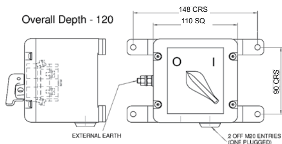
25A Die cast Aluminium Enclosure (A)
