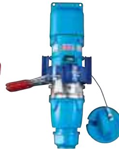
Padlocked in OFF position*
