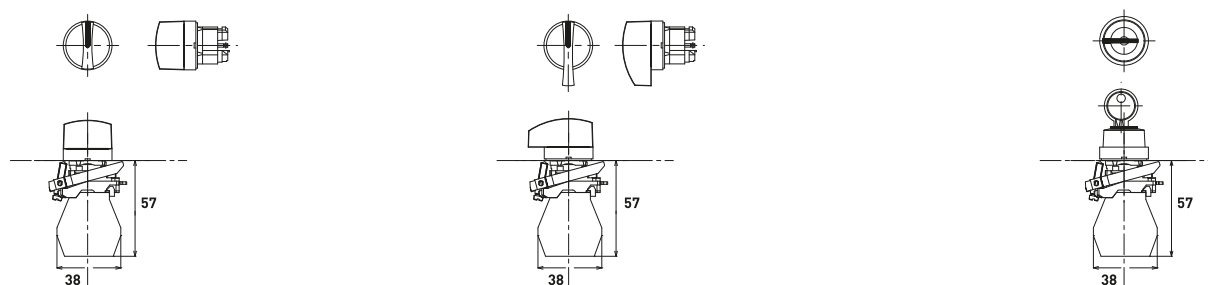
Selector switches with standard handle
