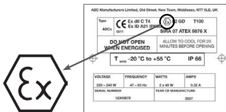
Figure 1 Typical ATEX equipment marking plate
