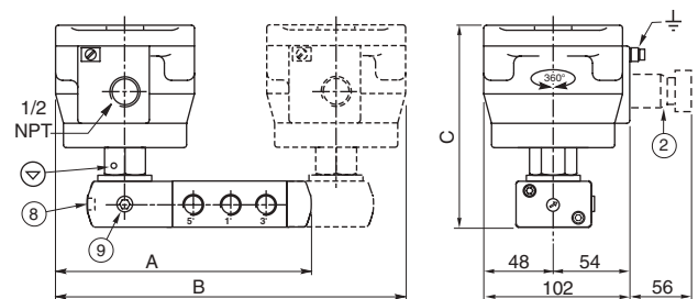
TYPE 04: Metal, epoxy coated / AISI 316L SS WP / WS: IEC 335 EM / WSEM: EN/IEC 60079-17+31
