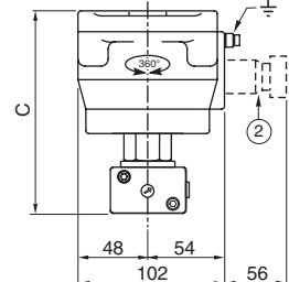
TYPE 04: Metal, epoxy coated / AISI 316L SS WP / WS: IEC 335 EM / WSEM: EN/IEC 60079-7+18+31
