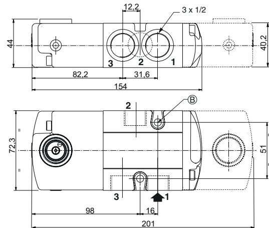
TYPE 02: Aluminium, epoxy coated / AISI 316L SS NF / WSNF: EN/IEC 60079-1, 60079-31
