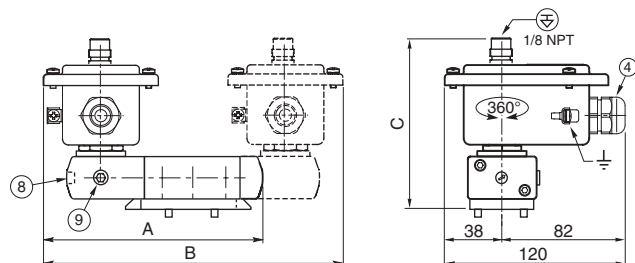
TYPE 11: Epoxy encapsulated EF: NEMA type 7, 9 / ICS-6 ANSI
