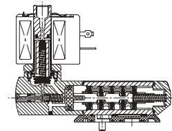
3/2 NC - 5/2 function
