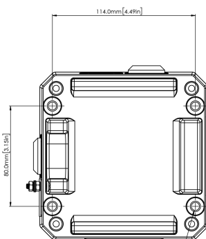
Ø 6.4mm [0.25in] MOUNTING HOLES 4 OFF
