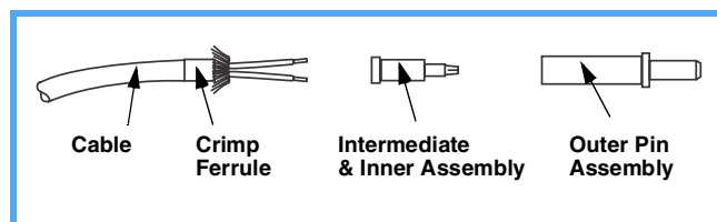
RCT (Reduced Component Twinax) Contact
