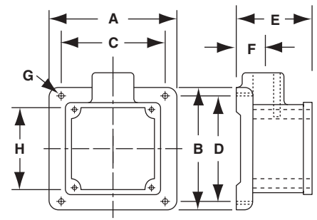
Form sizes 7-Z & 8-Z
