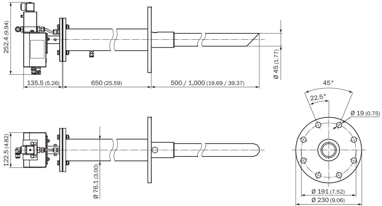
ZIRKOR200 analyzer unit with cooling protection tube
