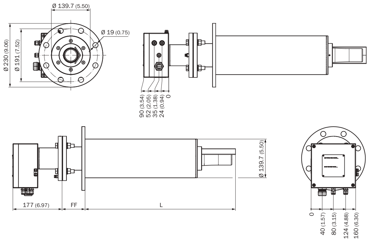
ZIRKOR200 Ex-D analyzer unit
