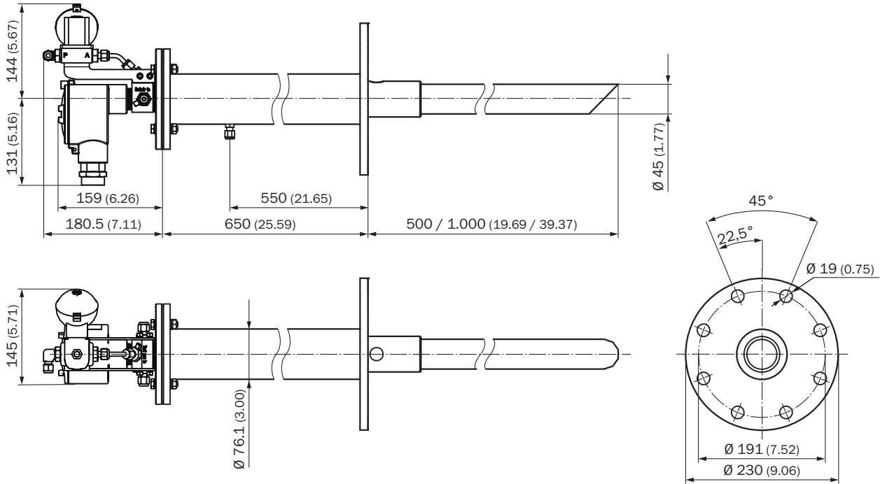
ZIRKOR200 Ex-G analyzer unit with cooling protection tube
