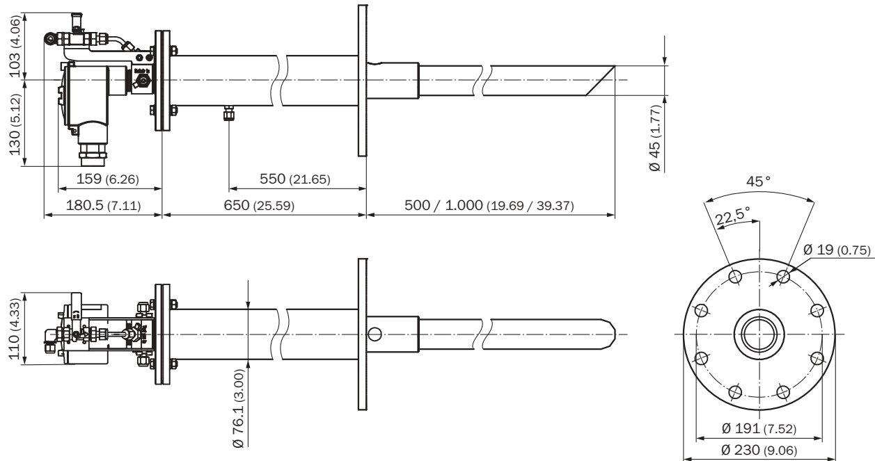
ZIRKOR200 Ex-G analyzer unit with manual valve and cooling protection pipe
