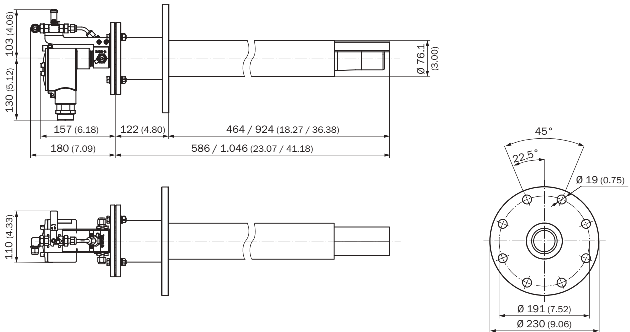
ZIRKOR200 Ex-G analyzer unit with manual valve
