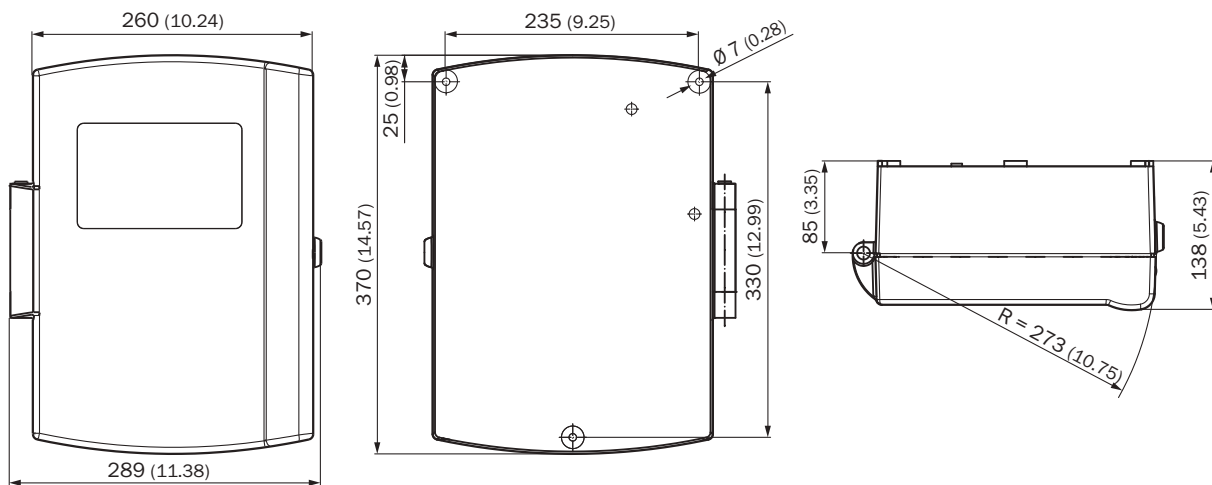
Control unit; cast metal housing
