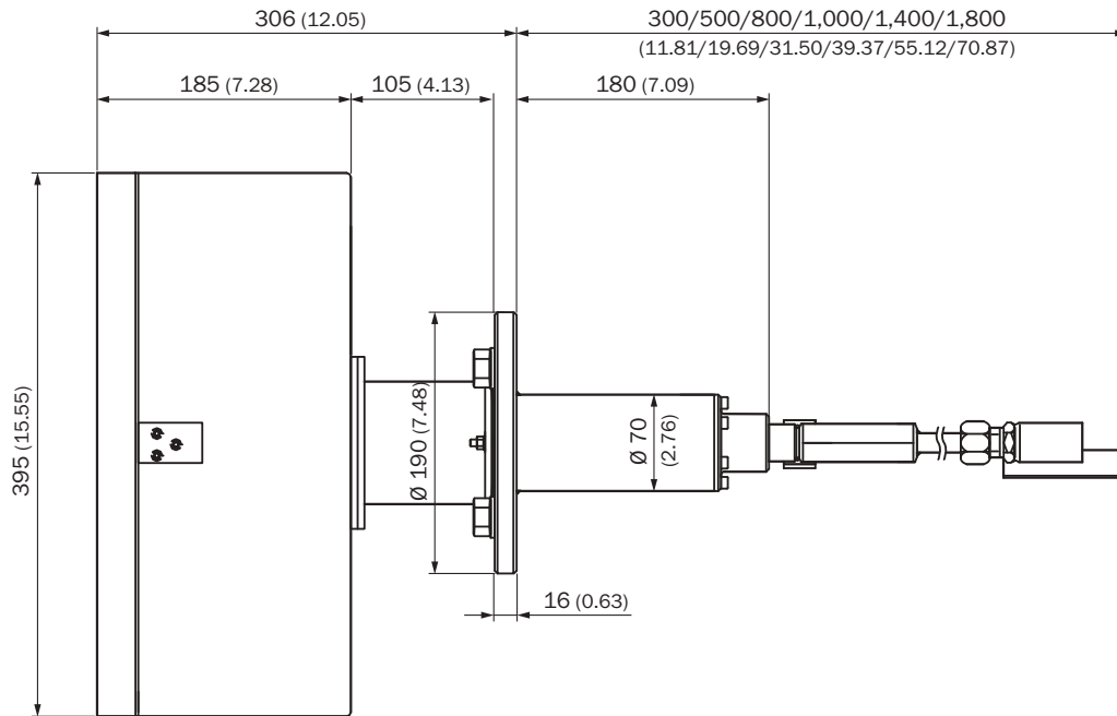
ZIRKOR302 analyzer unit
