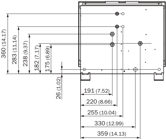
GMS840 design
