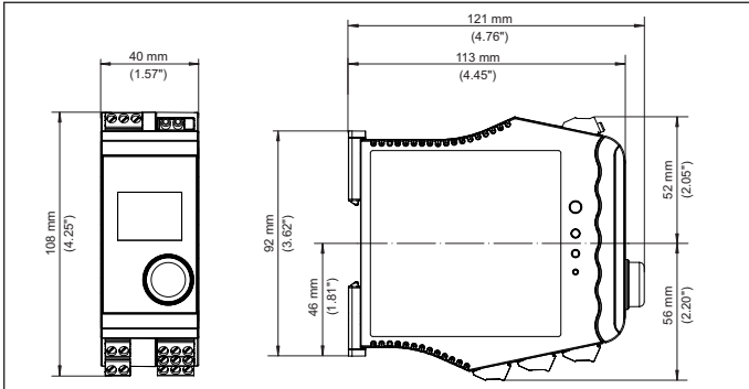
Fig. 16: Dimensions VEGAMET 141
