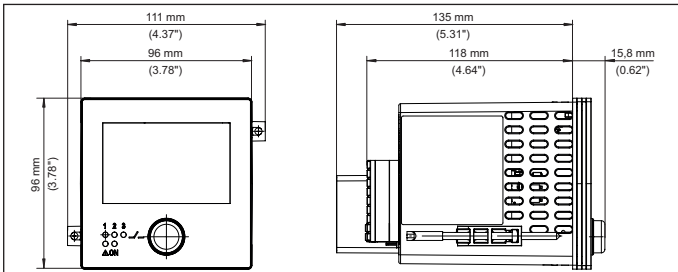
Fig. 18: Dimensions VEGAMET 341
