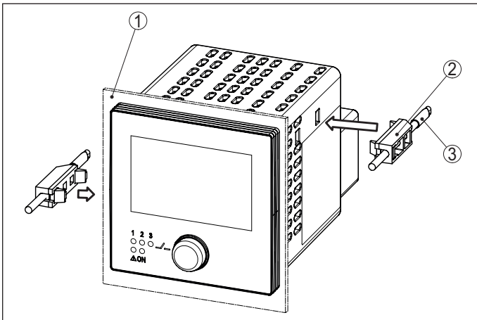
Fig. 2: Front panel mounting
