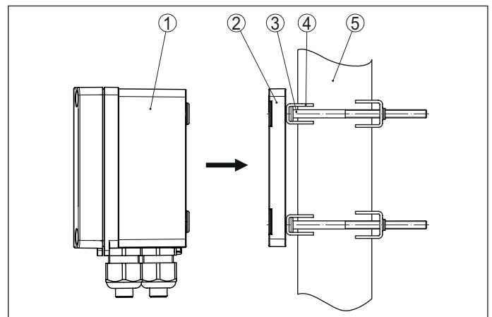
Fig. 5: Tube mounting
