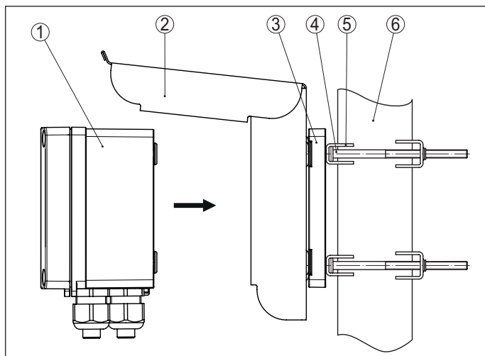
Fig. 6: Mounting sun protection with pipe mounting
