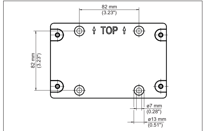
Fig. 3: Mounting plate for wall mounting (VEGAMET 841, 842)
