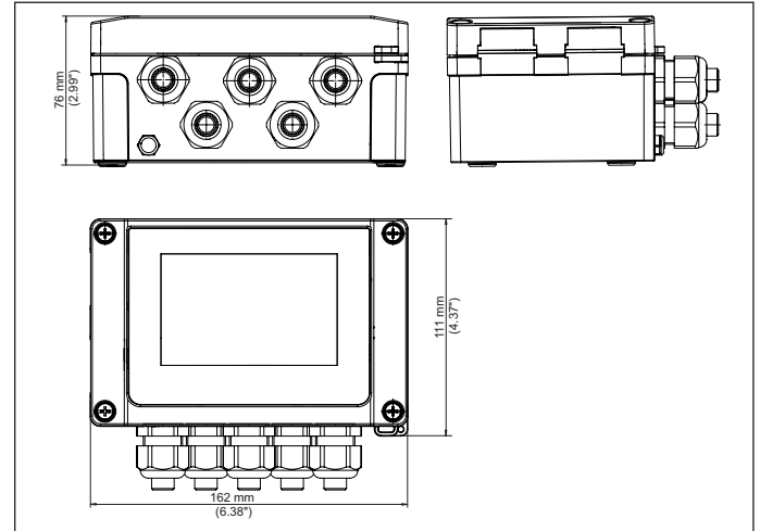
Fig. 20: Dimensions VEGAMET 841, 842
