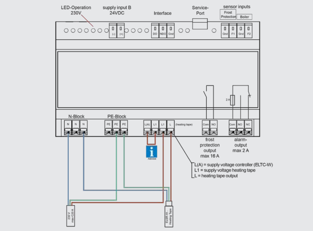
Wiring diagram: Heater and temperature controller connected on same feeding circuit
