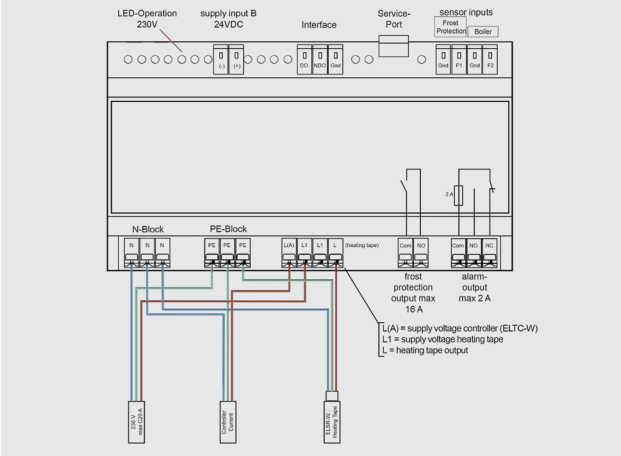
Wiring diagram: Separate feeders for controller device and heating circuit
