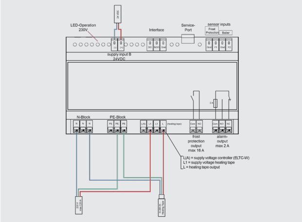
Wiring diagram: Separate 24 VDC supply
